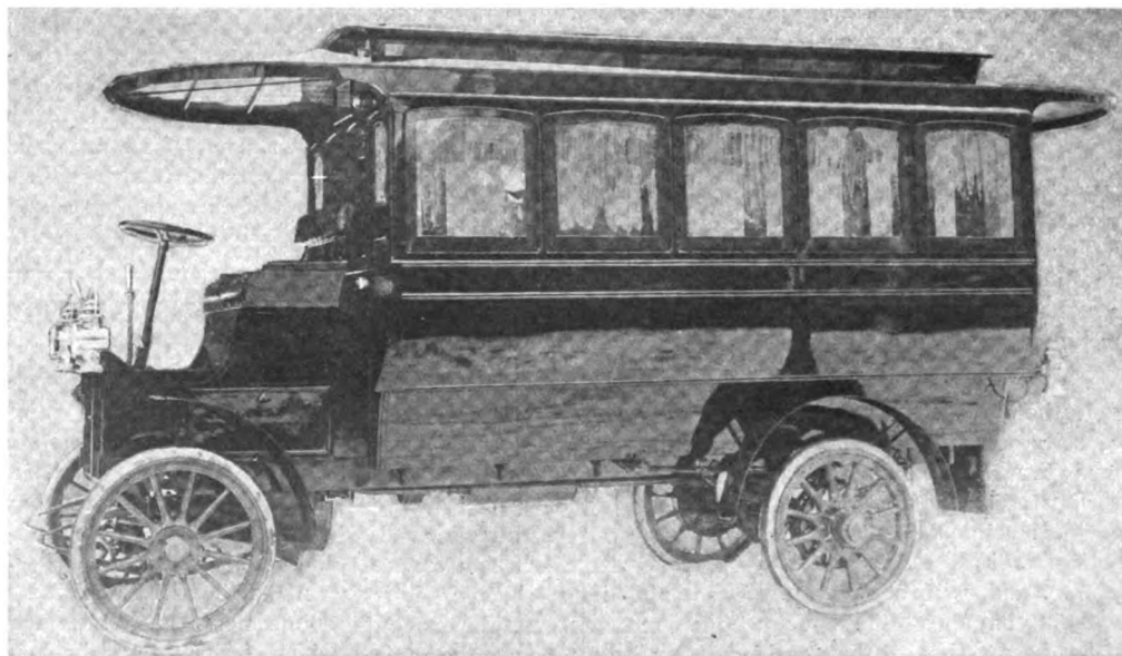
Franklin Air-Cooled 'Bus in Service on Sixteenth Street, Washington.
